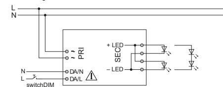
Collegamento DALI-PUSH DALI-PUSH diagram
